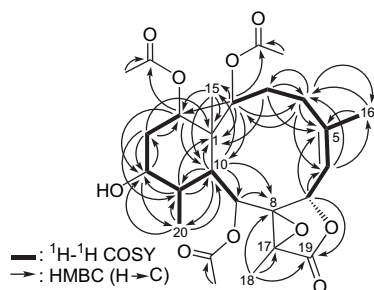
Figure 1. The 1 H– 1 H COSY and HMBC correlations of 1 .
