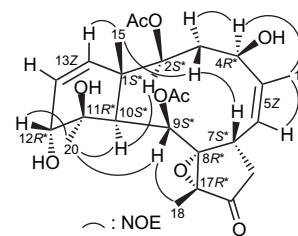
Figure 4. Selective NOESY correlations of 3 .
