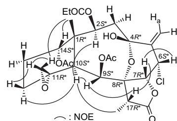
Figure 9. Selective NOESY correlations of 10 .
