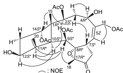
Figure 3. Selective NOESY correlations of 2 .
