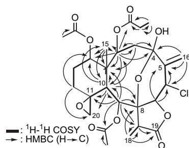
Figure 8. The ^1\text{H} – ^1\text{H} COSY and HMBC correlations of 10 .
