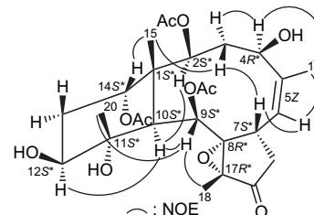
Figure 5. Selective NOESY correlations of 4 .
