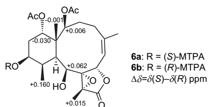
Figure 7. ^1\text{H} NMR chemical shift difference [ \delta(S)\text{-MTPA} - \delta(R)\text{-MTPA} ] of the MTPA esters of 6 .
