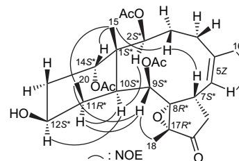
Figure 2. Selective NOESY correlations of 1 .
