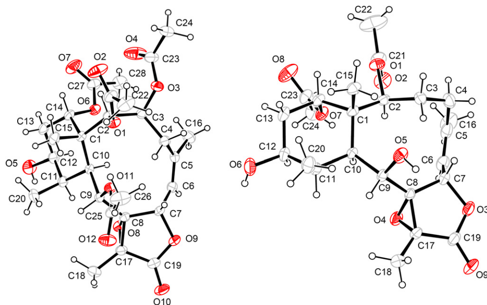
Figure 6. Computer-generated ORTEP plots of 5 and 6 showing the relative configurations.
